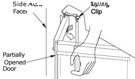
Figure 2 - Door Adjustment
