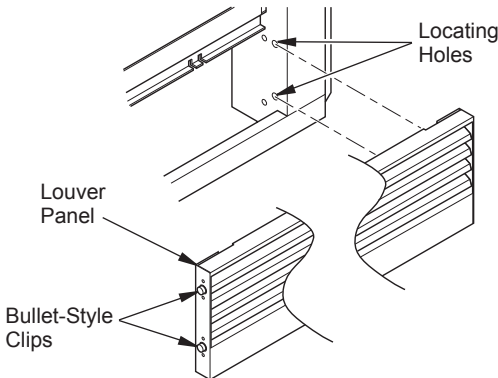
Figure 4 - Removing Louver Panel with Bullet-Style Clips (Direct-Vent Models)
