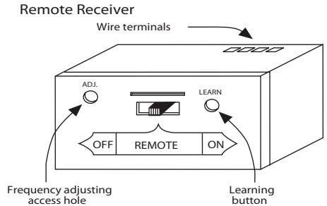
Figure 8: Adjusting the Receiver
