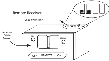
Figure 5: Remote Receiver
