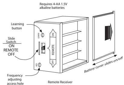
Figure 2: Remote Receiver
