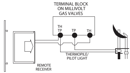
Figure 6: Millivolt Wiring Diagram
