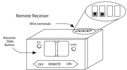
Figure 5: Remote Receiver
